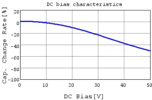
RCER71H104K0A2H03B C-DC bias capchange, 25.0
