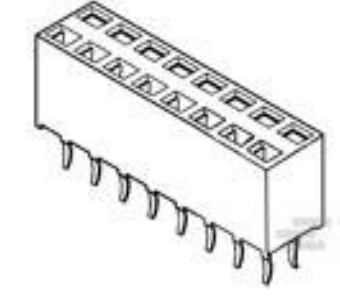
TE Part #215310-2 2X2P HV100 REC CON. TE, 8.5MM,TIN
